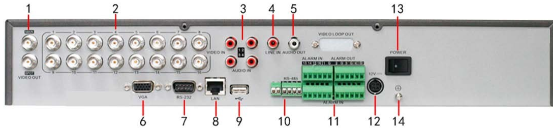
Figure 20. DS-7216HVI-ST/RW Rear Panel
