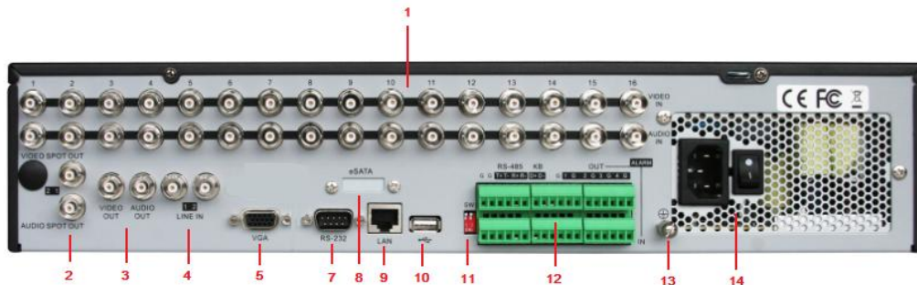
Figure 10. DS-9000/9100-S DVR Rear Panel Diagram
